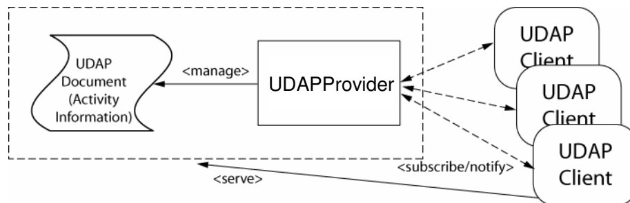
Figure 1 The figure shows the UDAP Provider in charge of a UDAP Document for an activity (represented by the dashed box) on a Grid. UDAP Clients concerned with that activity may subscribe to the UDAP Provider so that they can be notified of changes in the activity.
